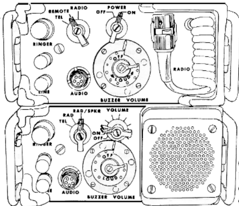
Figure F-14. Radio Set Control Group AN/GRA-39.
